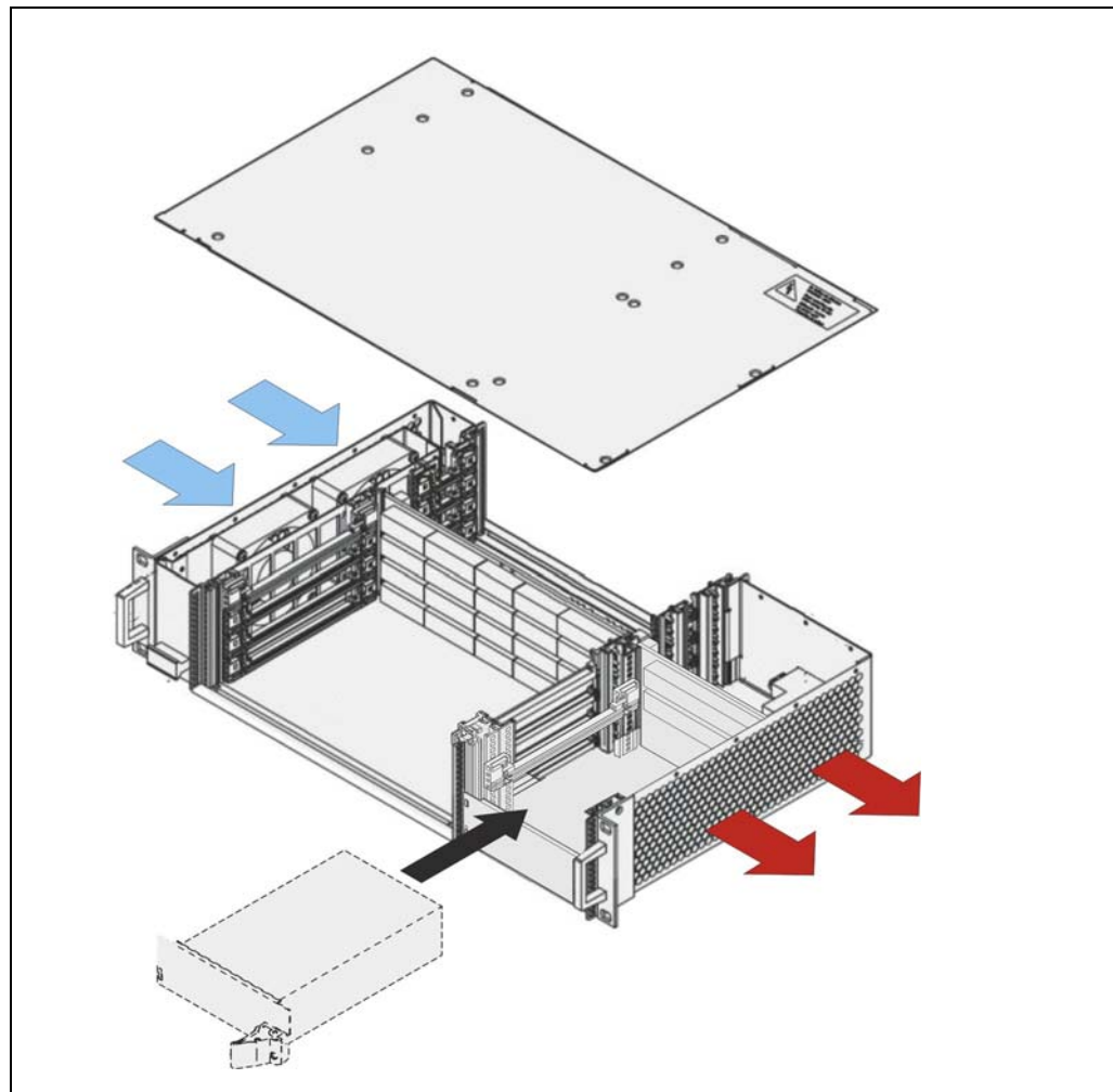
Figure 5: Air Flow
