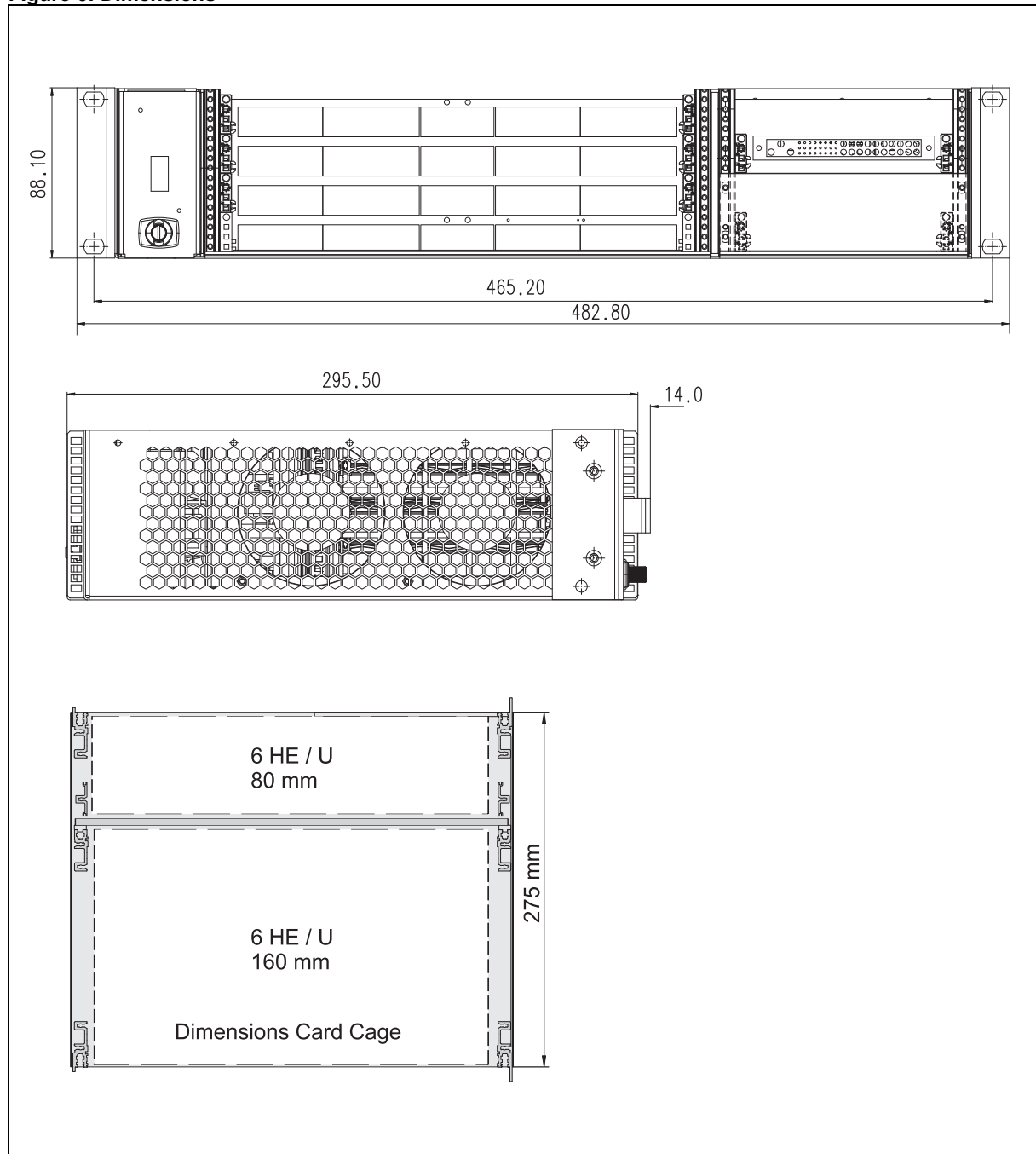
Figure 6: Dimensions
