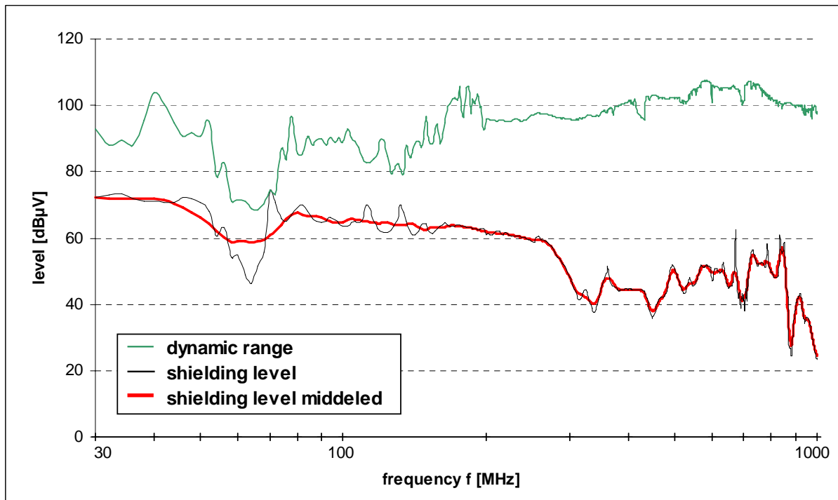
Fig. 6: Measurement results for direct radiation on LEFT-side of the EUT
