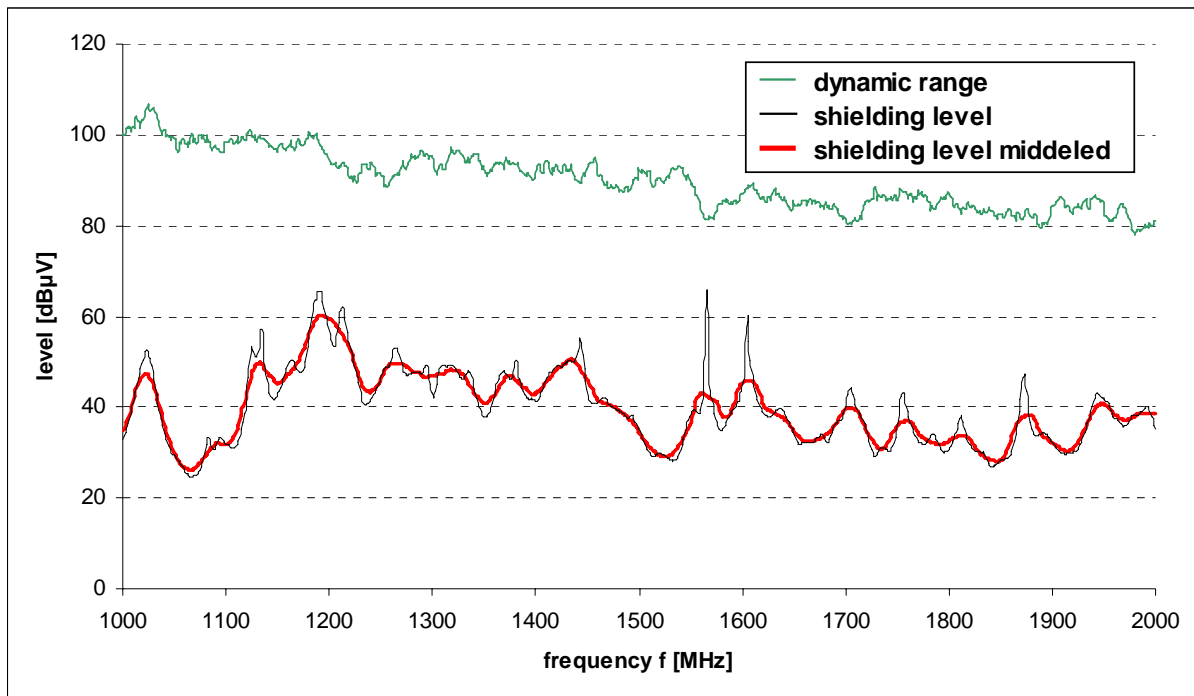
Fig. 11: Measurement results for direct radiation on BOTTOM-side of the EUT
