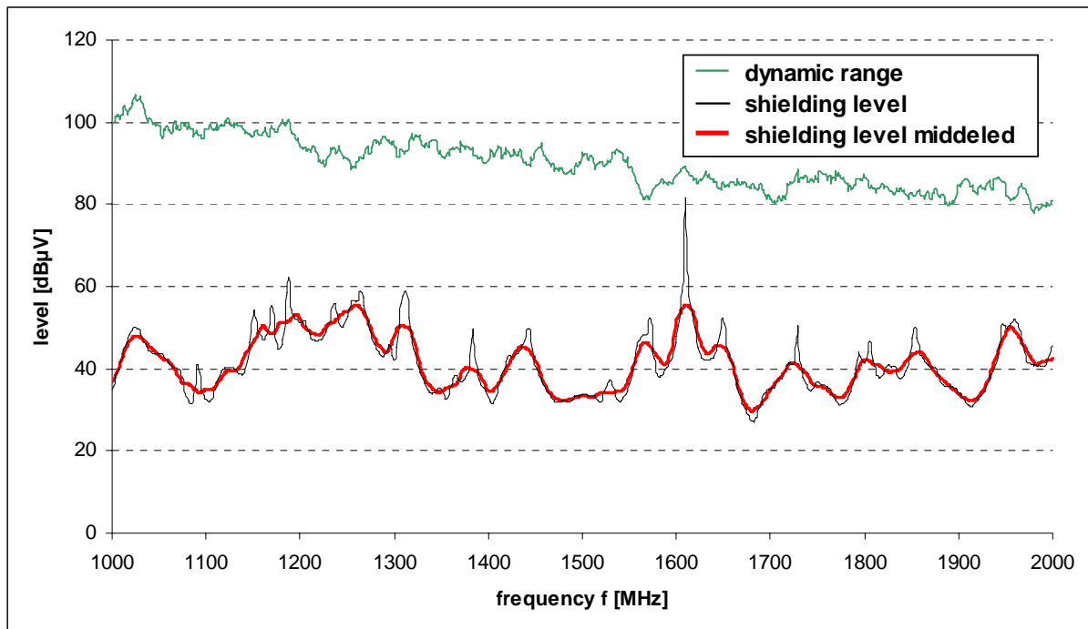
Fig. 9: Measurement results for direct radiation on TOP-side of the EUT
