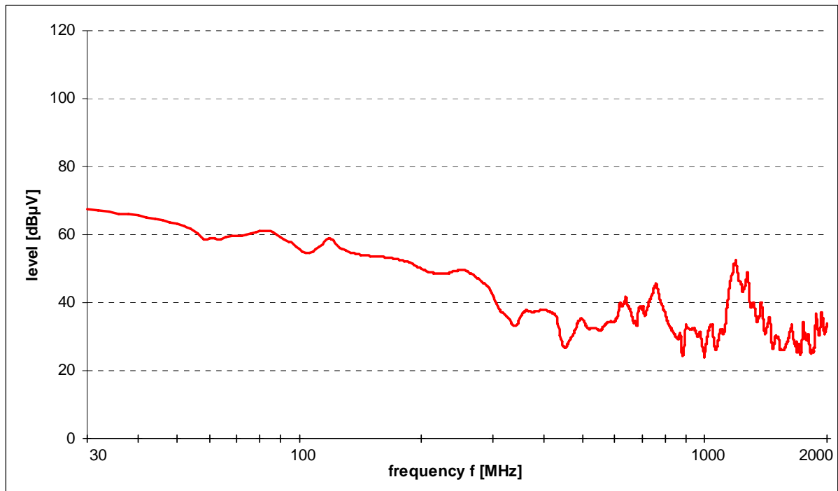
Fig. 13: Typical shielding effectiveness and worst case scenario of the EUT
