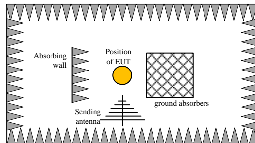
Fig. 2: Setup for 1 GHz – 2 GHz
