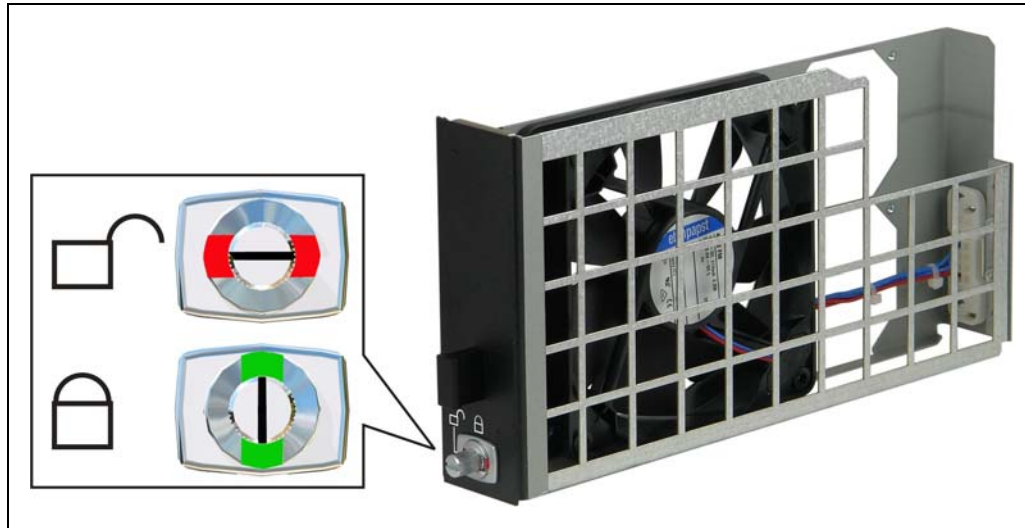
Figure 4: Fan Tray
