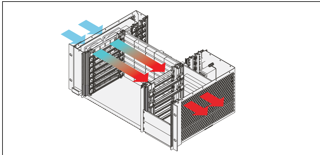
Figure 5: Airflow
