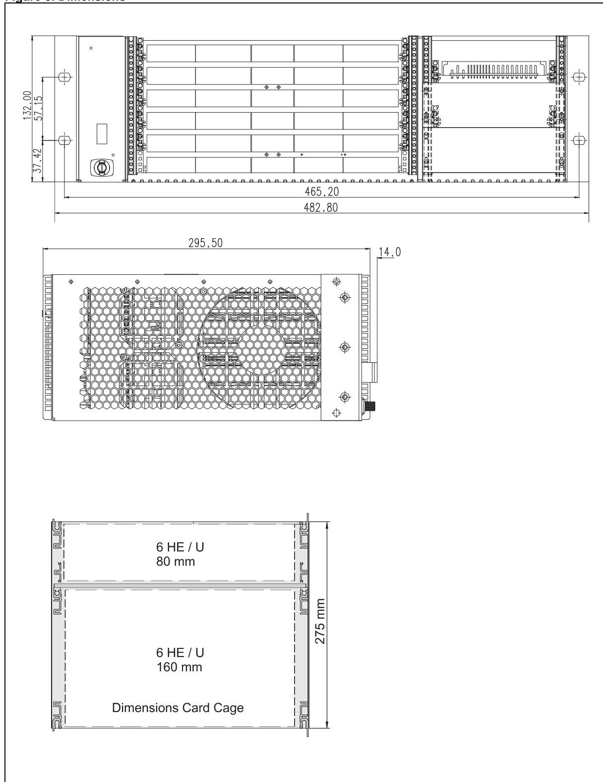
Figure 6: Dimensions
